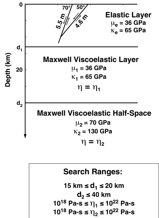
Figure 4. Fault and rheological model used for the Hebggen Lake earthquake and fault area. Four parameters, the depths, d_1 and d_2 , and viscosities, \eta_1 and \eta_2 , of two viscoelastic strata were evaluated by a Monte Carlo search. Fault source parameters are from Doser [1985]. The shear modulus, \mu , and the bulk modulus, \kappa , were based on the average crust and upper mantle P -wave velocities of the Hebggen Lake-Yellowstone region [Smith et al. , 1989]. The densities are 2800, 3100, and 3400 \text{ kg/m}^3 for the elastic layer, viscoelastic layer, and half-space, respectively.
