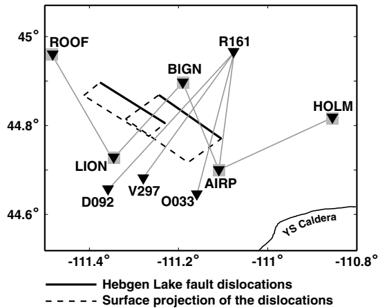
Figure 3. Geodetic stations and baselines used for rheologic modeling. Dashed rectangles show the surface projections of the 1959 Hebggen Lake fault dislocations [Barrientos et al. , 1987].
